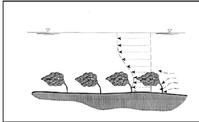
Figure 7: Reconfiguration of vegetation shape due to water flow and influence of vertical flow velocity profile.
