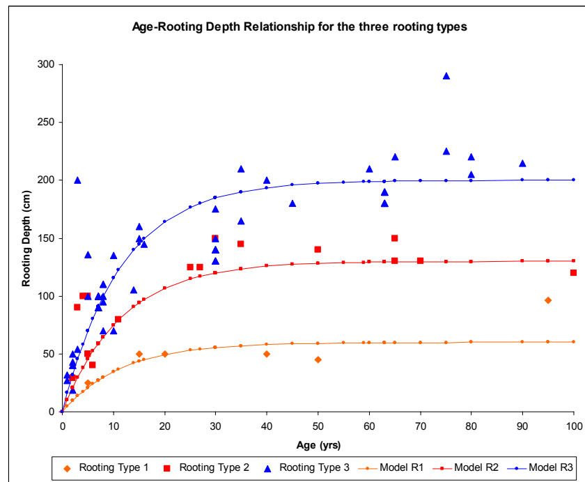
Figure 2: Age-rooting depth relationship for the three rooting types based on the regrouped species-specific data (obtained from the literature) with the corresponding 'theoretical' models.
