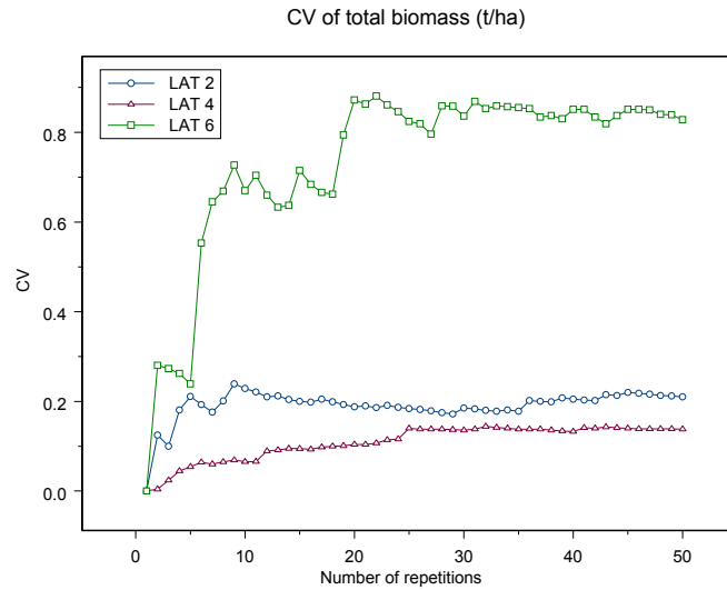
Figure 10: Development of the coefficient of variation (CV) in relation to the number of model repetitions for LAT 2, 4 and 6 after 30 years of simulation.
