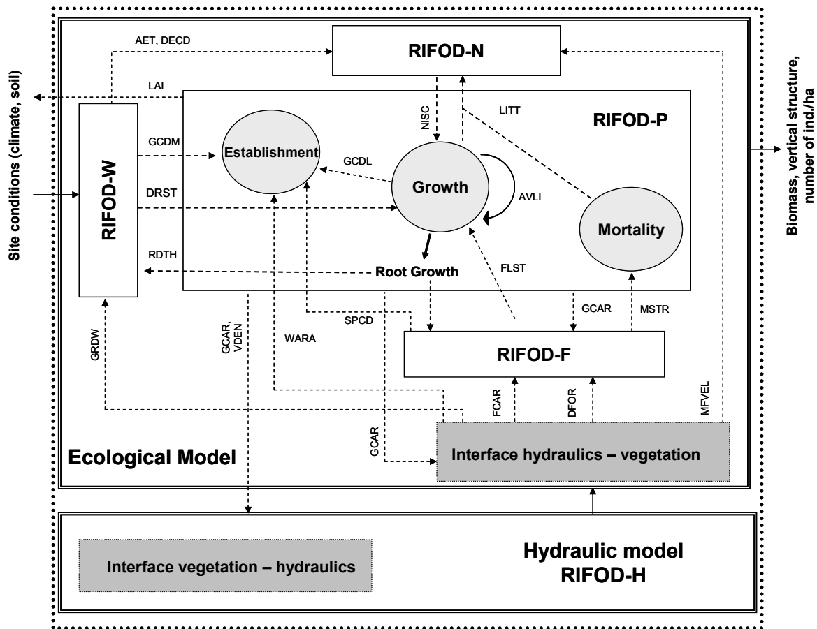
Figure 2: Conceptual representation of the ecological model structure with the modules (RIFOD-W, RIFOD-N, RIFOD-F) calculating the environmental stress and their influence on the population dynamics module RIFOD-P and the variables exchanged between these modules. RDTH; rooting depth, GCDM, moisture germination conditions, GCDL; light germination conditions, DRST; drought stress ( i.e. soil moisture growth factor; SMGF), NISC; nitrogen scarcity ( i.e. soil nitrogen growth factor; SNGF), LITT; litter production, GEAR; geometrical plant characteristics ( e.g. crown height), MSTR; mechanical stress, SPCD; sprouting conditions, FLST; physiological flooding stress ( i.e. flooding growth factor; FLGF), FCAR; flooding characteristics ( e.g. flooding duration), DFOR; drag force, GRDW; groundwater level, VDEN; vegetation density, MARA; wetted area. AVLI; light availability, MVEL; maximal flow velocity, LAI; leaf area index, AET; actual evapotranspiration, DECD; conditions of denitrification.
