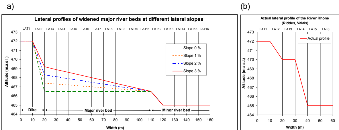
Figure 17: Lateral half-profiles of the River Rhone: (a) lateral half-profiles for the river widening variants at a major river bed width of 90 m, (b) actual half-lateral profile of the River Rhone at Riddes (Valais).
