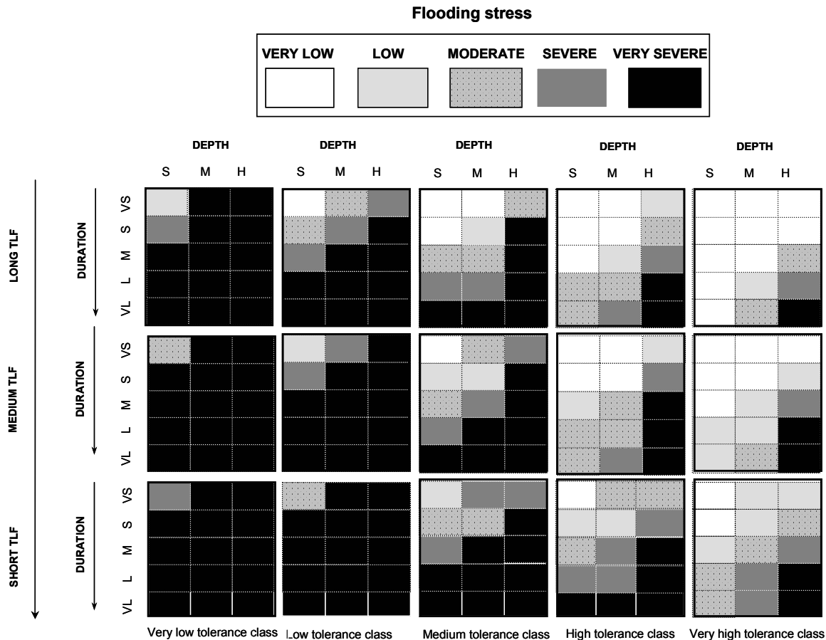
Figure 2: Developed fuzzy rules for the five flooding tolerance classes to model flooding growth stress by increasing flooding depths (shallow/soil submersion, S; medium/partial submersion, M; high/complete submersion, H), TLF's (short, medium, long) and duration (very short, VS; short, S; intermediate, M; long, L; very long, VL).
