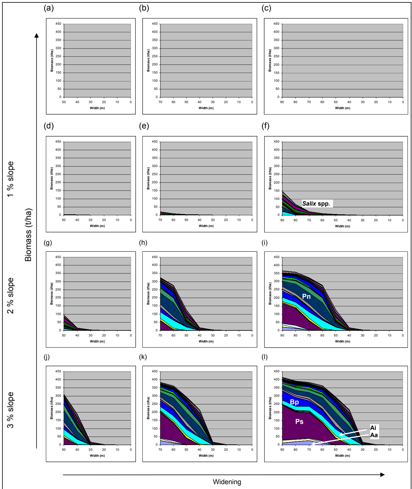
Figure 18: Lateral species-specific biomass distribution (t/ha) after 120 years of simulation at different major river bed widths (m) and lateral slopes (%). PS; Pinus sylvestris , Ai; Alnus incana , Aa; Abies alba ; Bp; Betula pendula , Pn, Populus nigra , Salix spp. ; Salix eleagnos , Salix daphnoides .
