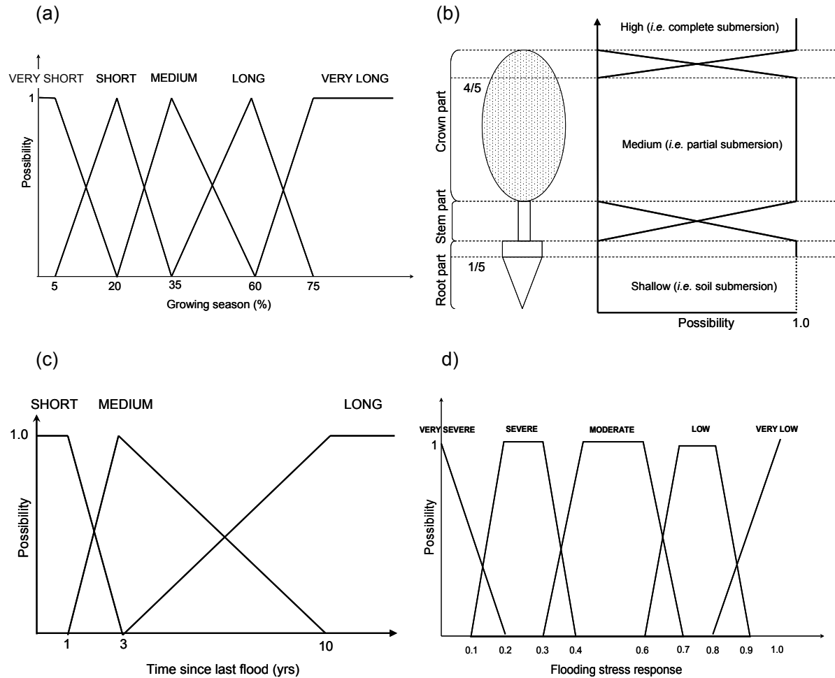
Figure 1: Membership functions for (a) flooding duration (very short, short, medium, long, very long duration), (b) flooding depth (high, medium, shallow flooding depth), (c) time since last flood (short, medium, long time since last flood) and (d) flooding stress response (very severe, severe, moderate, low, very low flooding stress).
