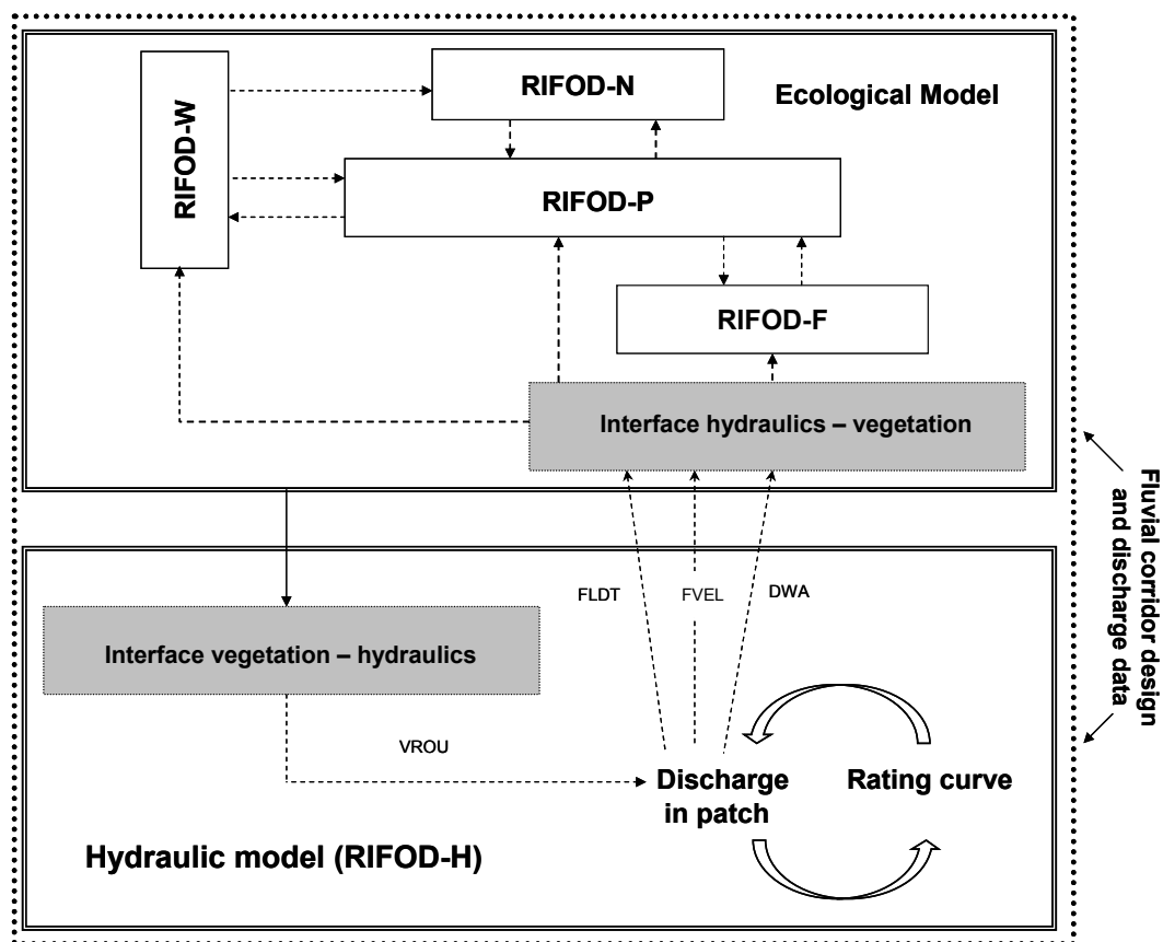
Figure 6: Conceptual representation of the hydraulic model and the coupling to the ecological model. FLDT; flow depth (m), FVEL; flow velocity (m/s), DWA; daily wetted area, VROU; vegetation roughness.
