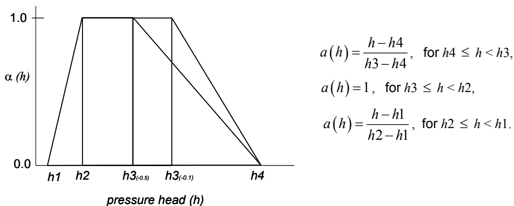
Figure 3: Reduction function \alpha(h) versus pressure head ( h ).
