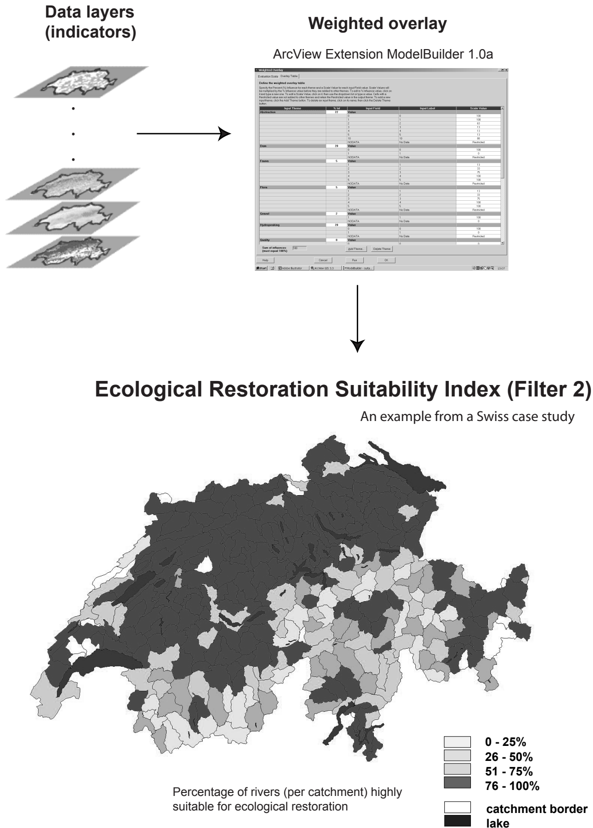
Figure 2. MCDM-GIS modelling
