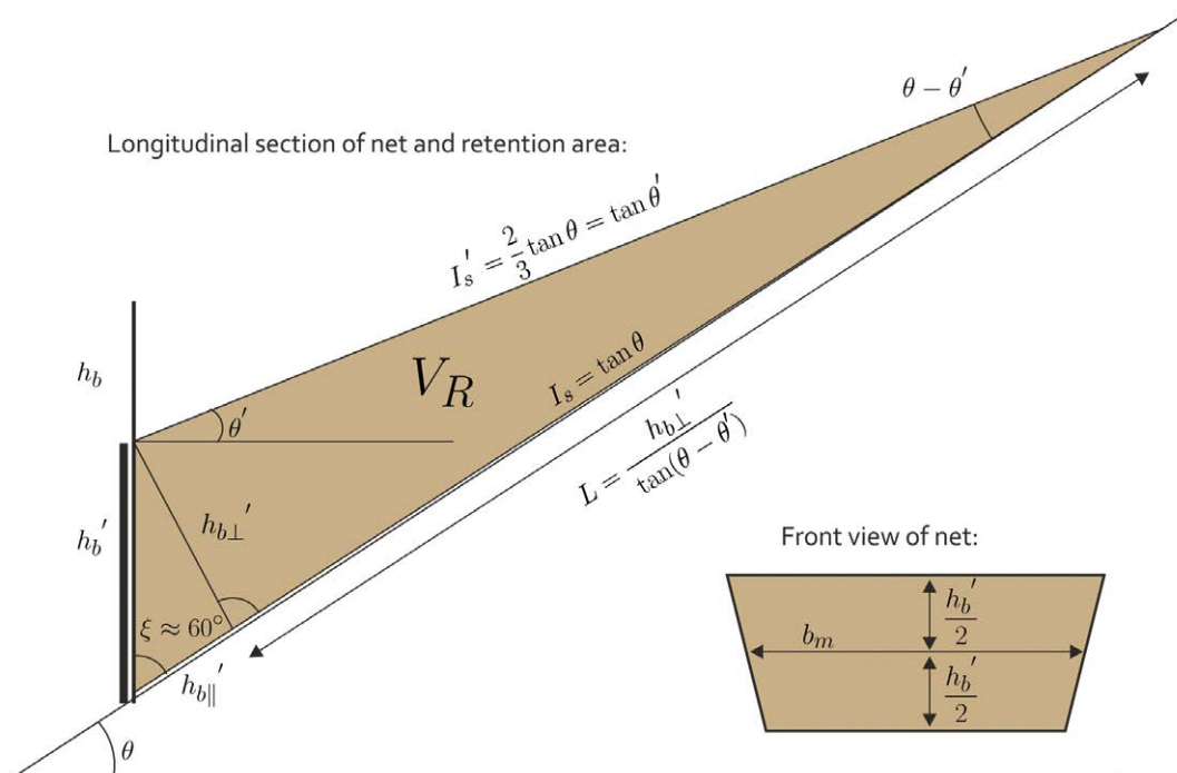
Fig. 5. Longitudinal section of torrent and front view of the net. Figure according to [36].
