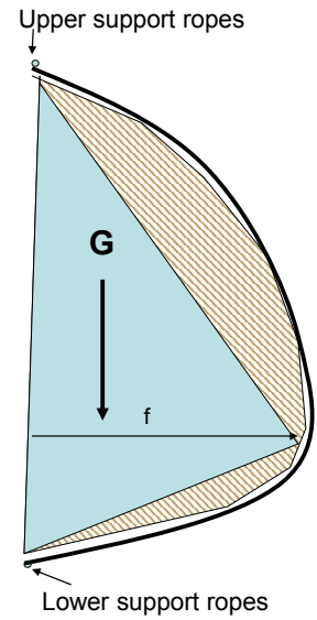
Fig. 24. Net deflection and self-weight of the net's belly. Figure according to [36].
