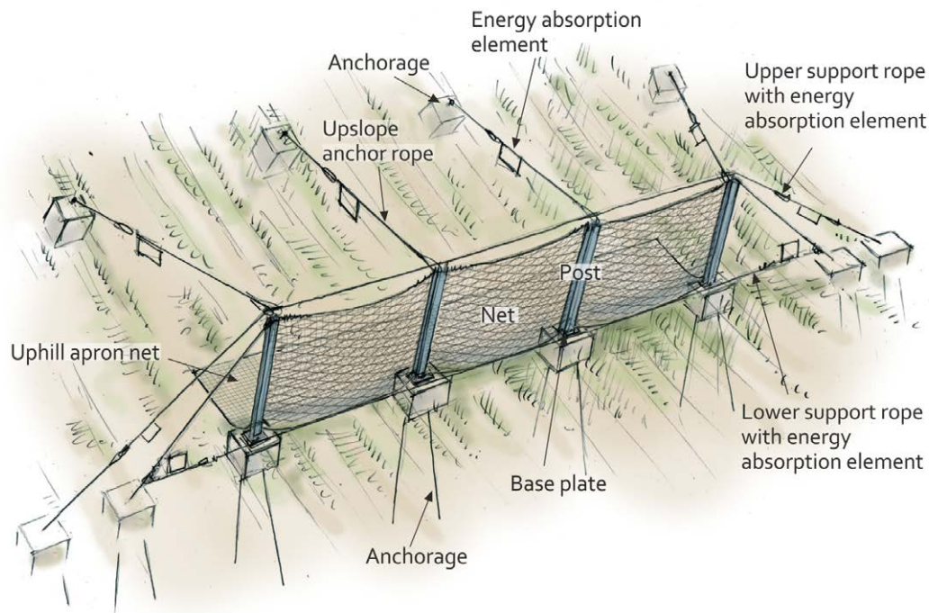
Fig. 2. Schematic view of the components and arrangement of a hillslope debris flow protection net, based on [12].
