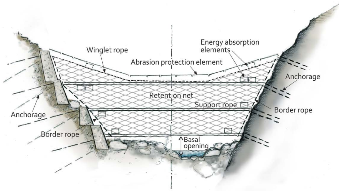
Fig. 1. Schematic view of the components and arrangement of a debris flow protection net for narrow, V-shaped channels, based on [12].
