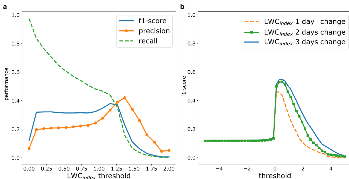
Figure 9. Performance statistics for two nowcast models, where (a) absolute values of the LWC_{index} and (b) temporal changes of LWC_{index} were used to predict avalanche days. A day is considered AvD if LWC_{index} \geq a specific threshold (x-axis), nAvD otherwise. In (b), negative (resp. positive) threshold values correspond to decreasing (resp. increasing) of LWC_{index} .
