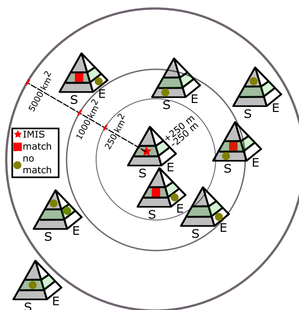
Figure 3. Schematic representation of how observed wet-snow avalanches on south facing slopes (red squares) were linked to input features derived from SNOWPACK simulations on a virtual south-facing slope at the location an AWS (station; red star). The pyramids represent different elevation bands and aspects for each observed avalanche and the virtual slopes at the station. The elevation bands show the \pm 250 m tolerance band. The circles represent the borders of areas surrounding the station. Green dots represent avalanches not assigned to the station because they did not satisfy the elevation and/or aspect criteria.
