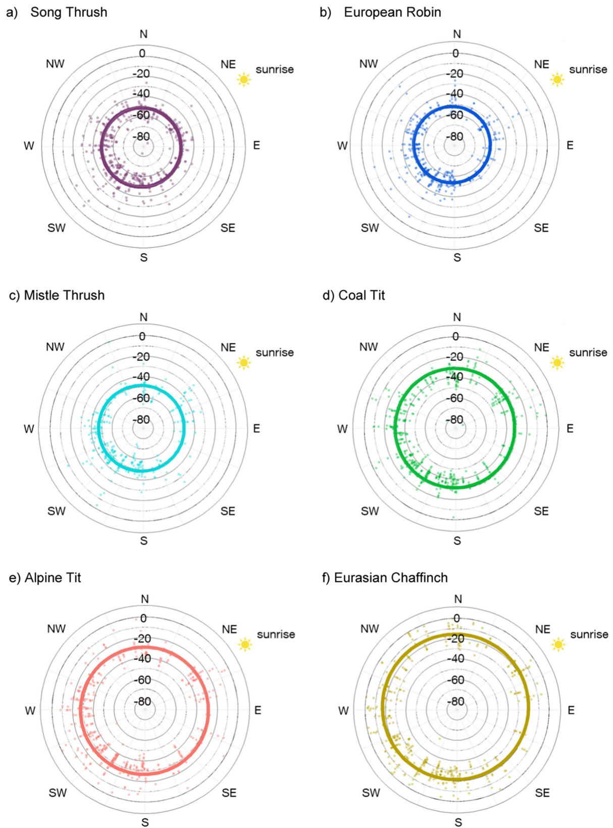
Fig. 3 Start of dawn singing in relation to aspect of a location. Black circles represent the time before sunrise in minutes (0 is sunrise and -60 is 1 h before sunrise). Coloured lines are estimates for the different species based on the GLMM. The symbol of the sun shows the angle of sunrise
