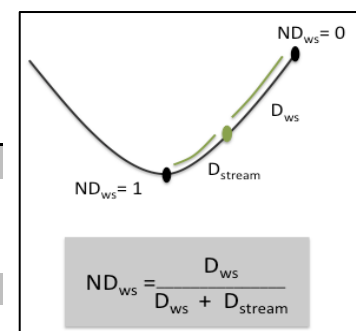
Fig. 5.1: Calculation of the normed distance (ND) to the watershed (ws).
