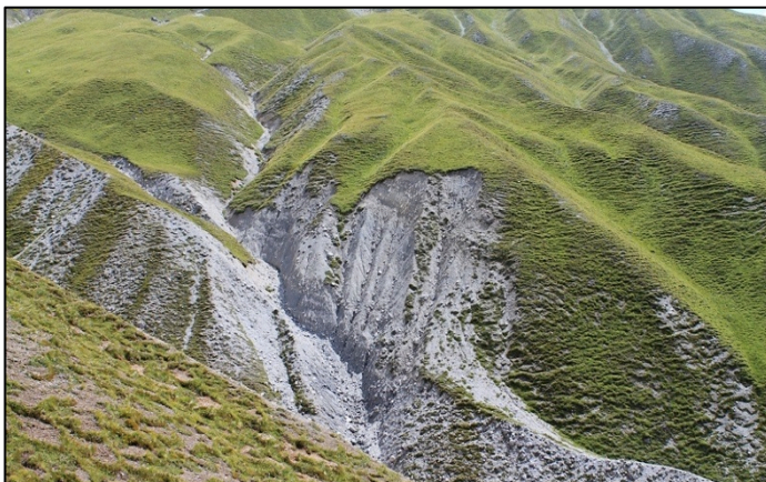
Fig. 2.8 (top): Moraine deposits in the upper Val dal Botsch, reworked by rill erosion and cryogenic creep resulting in the formation of garlands (Girlandenrasen). Fig. 2.9 (right): Alluvial deposits with large inputs of gravitational hillslope processes in Val Müschauns.
